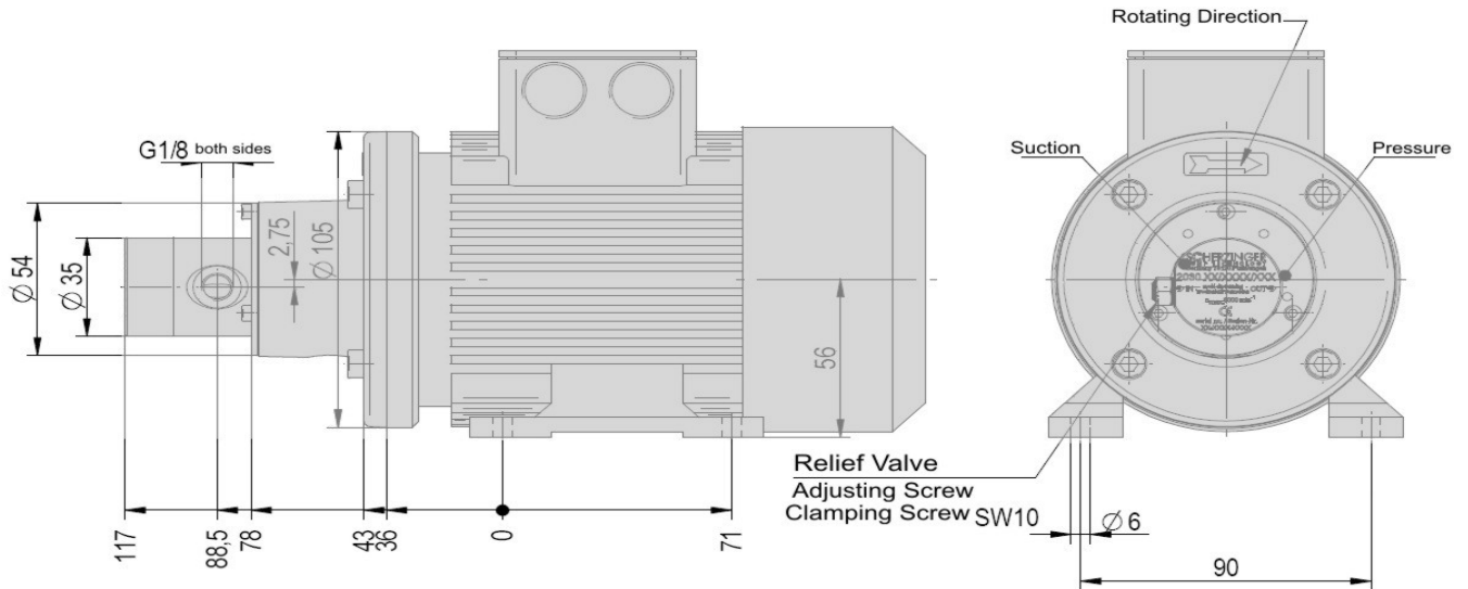
Typical dimensions of pump type 2030-016-B-DM06-2
