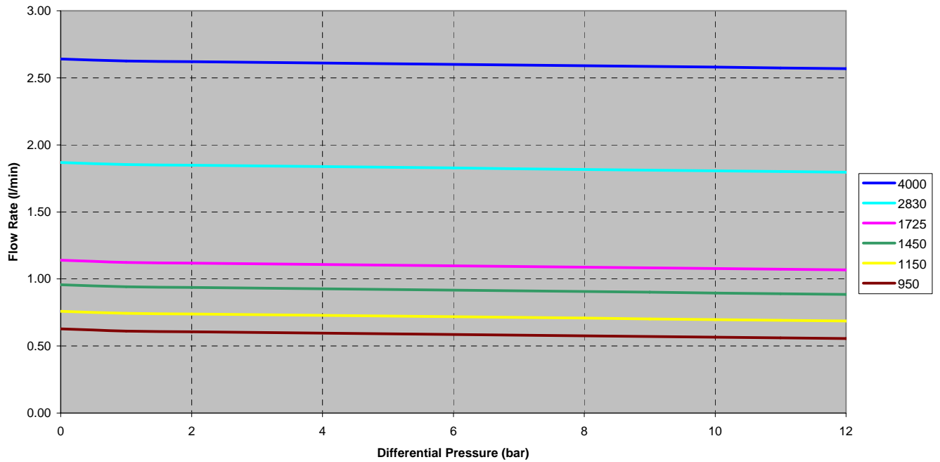
Pump Head 3030-070 measured with oil 100mPas
