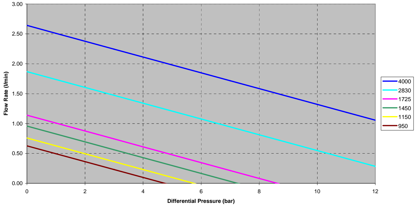
Pump Head 3030-070 measured with water 1mPas
